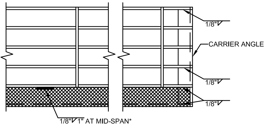
ON TREADS OVER 9-3/4" WIDE, WELD END OF CENTER BAR ALSO
