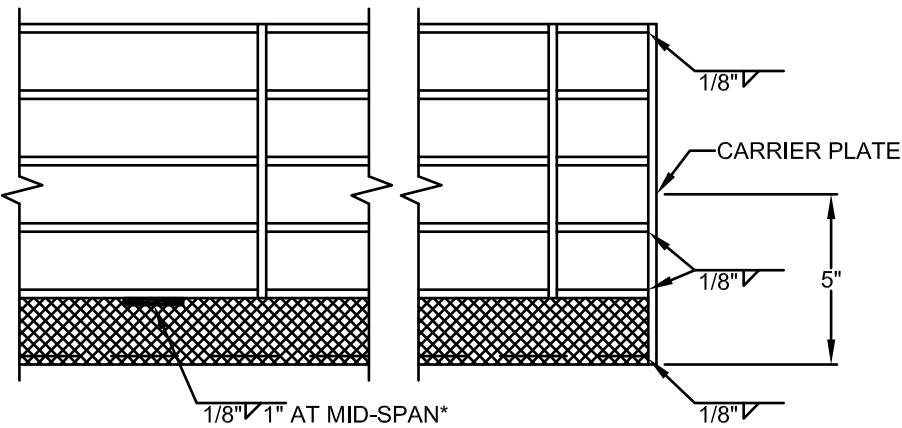
WHEN CARRIER PLATES ARE USED, THE BEARING BARS AND THE NOSING IN THE FRONT FIVE INCHES SHALL BE WELDED TO THE CARRIER PLATE AS SHOWN.
